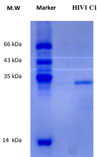
Figure- SDS PAGE Analysis
